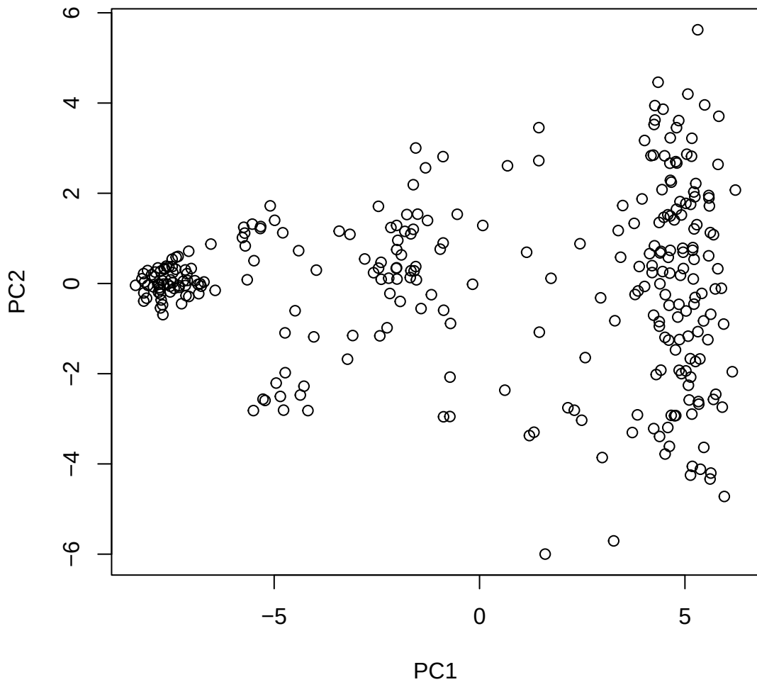
Window ID 81 NC_044051.1 (4)
