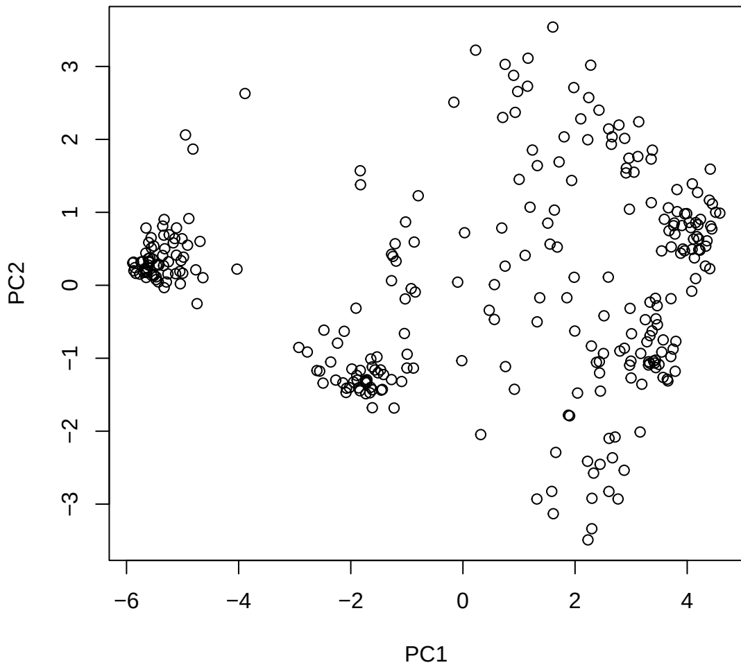
Window ID 92 NC_044051.1 (4)
