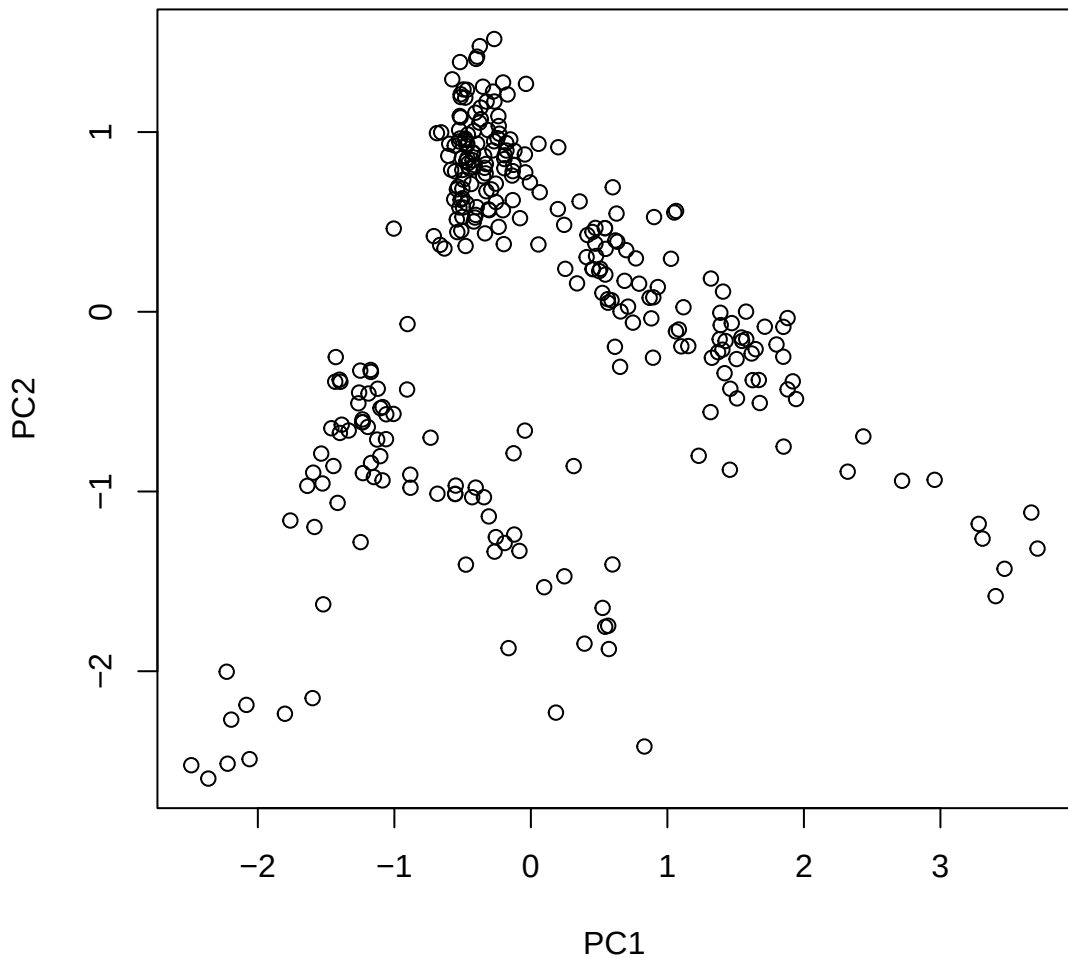
Window ID 97 NC_044051.1 (4)
