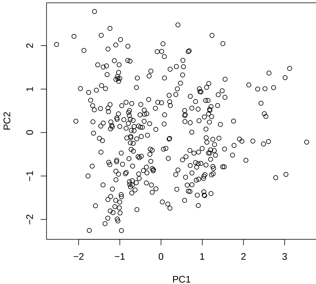
Window ID 98 NC_044051.1 (4)
