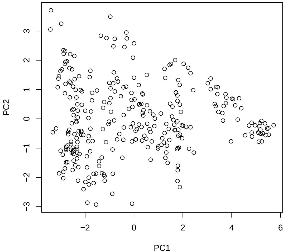
Window ID 130 NC_044053.1 (6)
