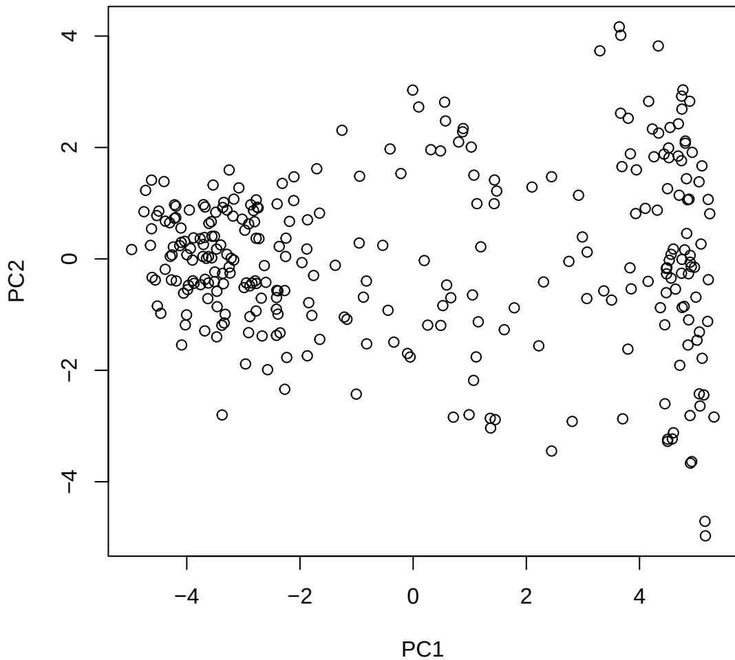
Window ID 134 NC_044053.1 (6)
