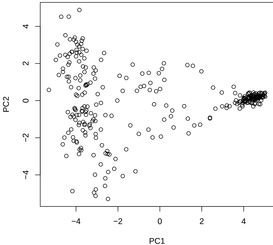
Window ID 135 NC_044053.1 (6)
