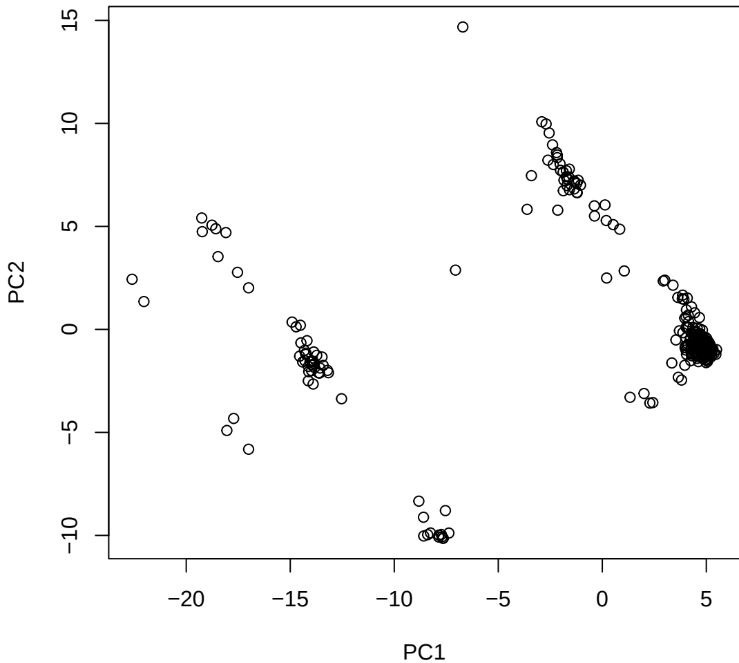
Window ID 137 NC_044053.1 (6)
