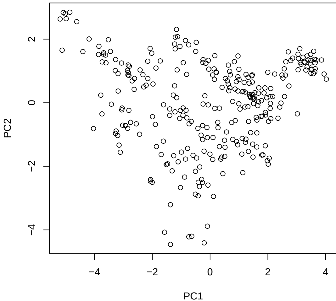
Window ID 149 NC_044053.1 (6)
