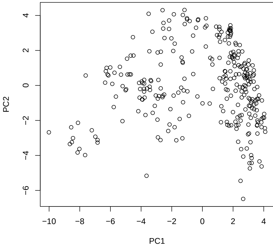
Window ID 179 NC_044054.1 (7)
