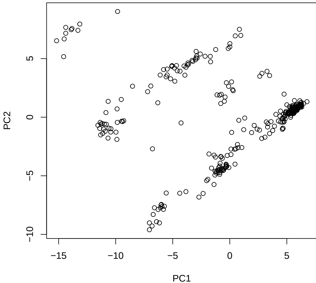
Window ID 180 NC_044054.1 (7)
