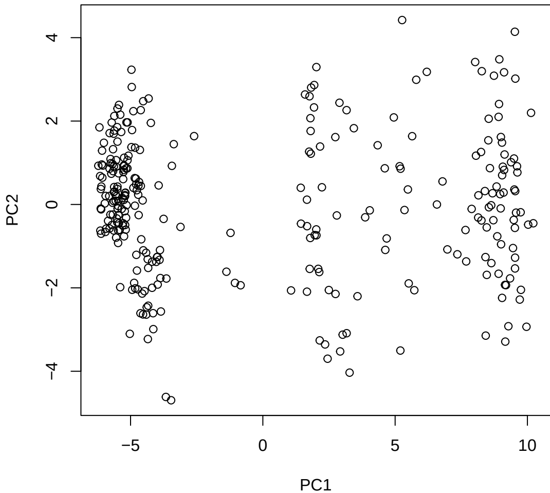
Window ID 187 NC_044055.1 (8)
