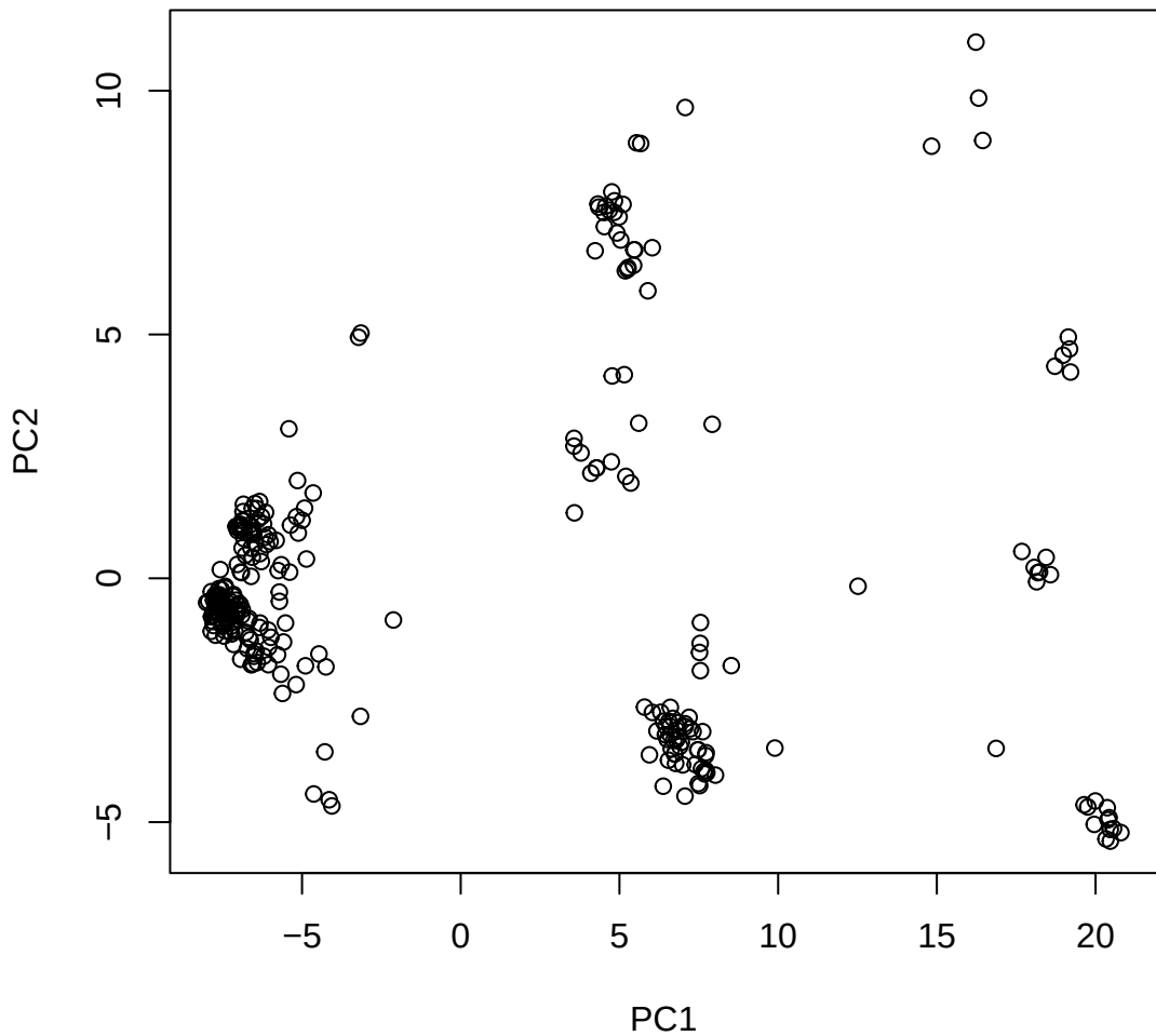
Window ID 197 NC_044055.1 (8)
