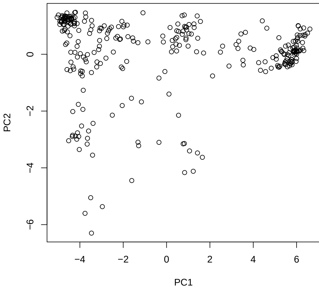
Window ID 198 NC_044056.1 (9)
