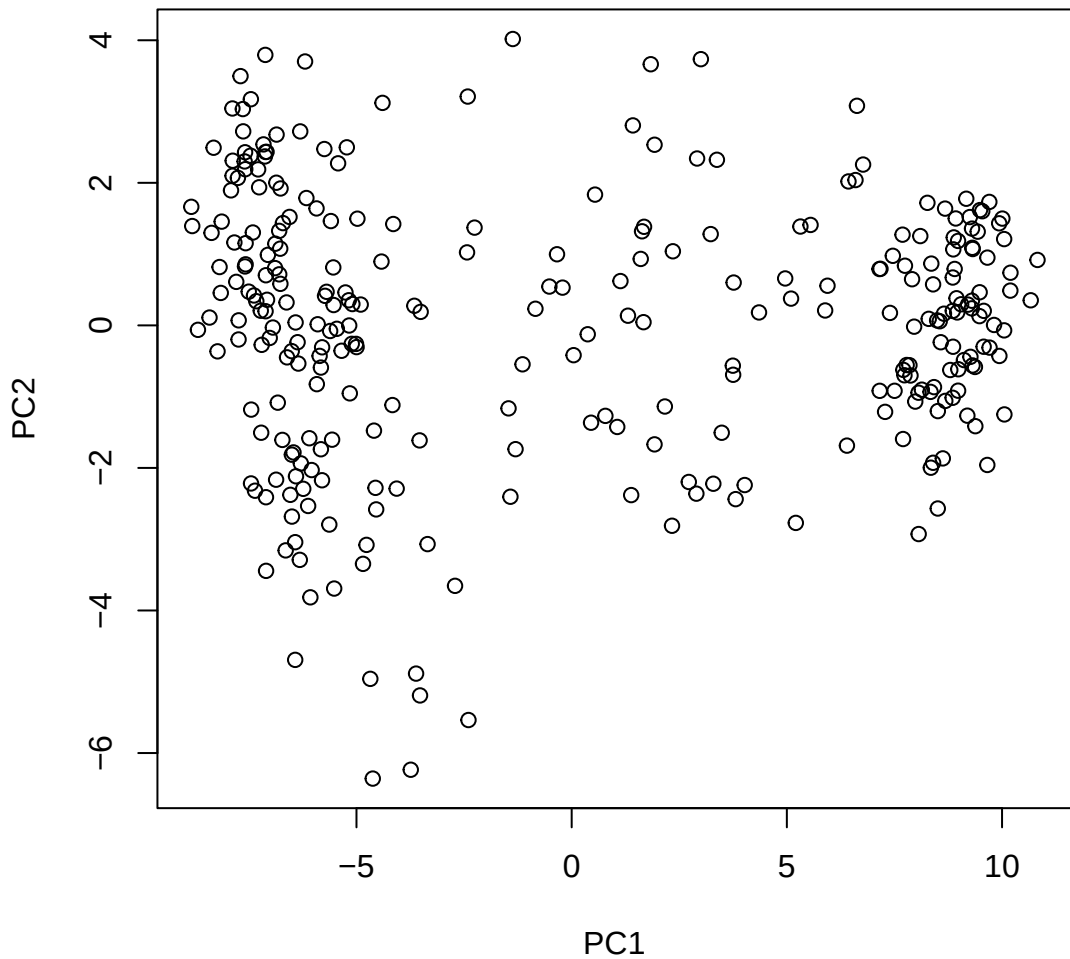
Window ID 209 NC_044056.1 (9)
