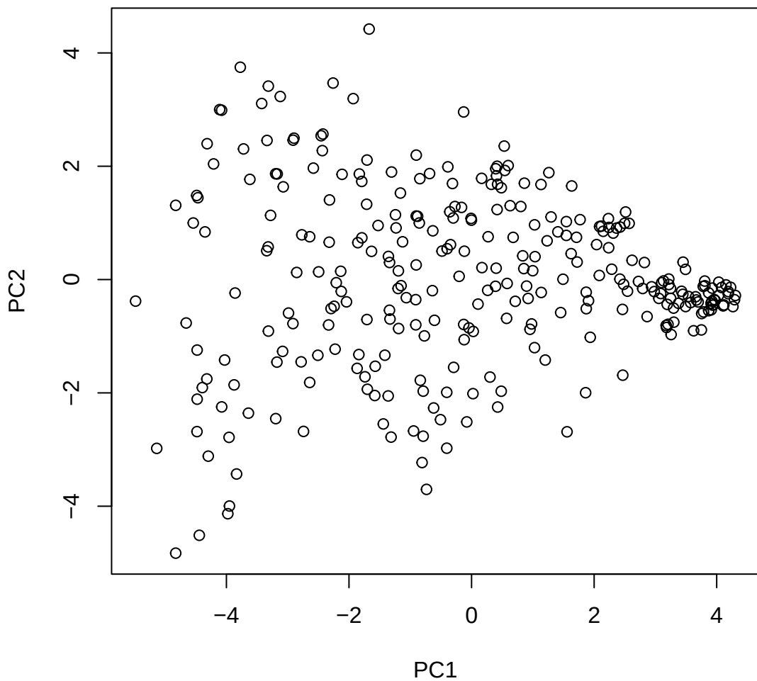
Window ID 211 NC_044056.1 (9)
