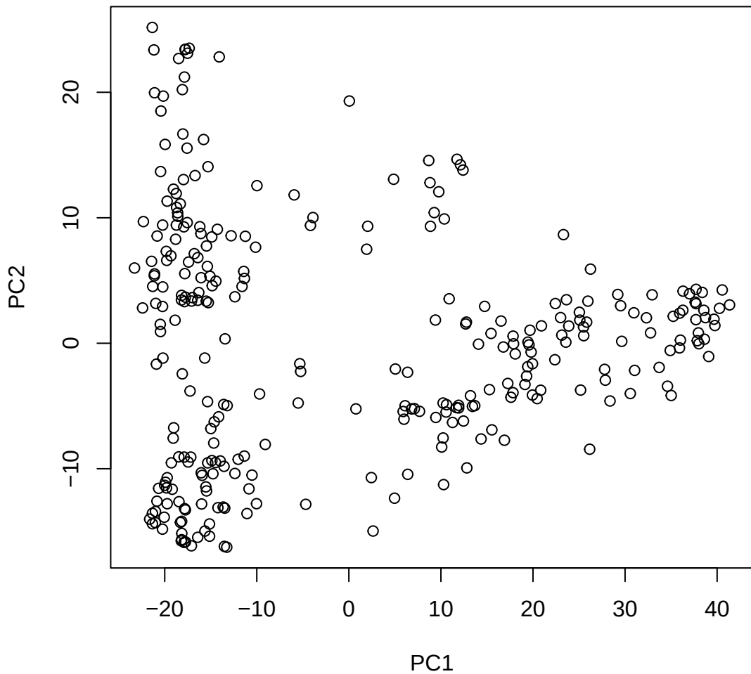
Window ID 212 NC_044056.1 (9)
