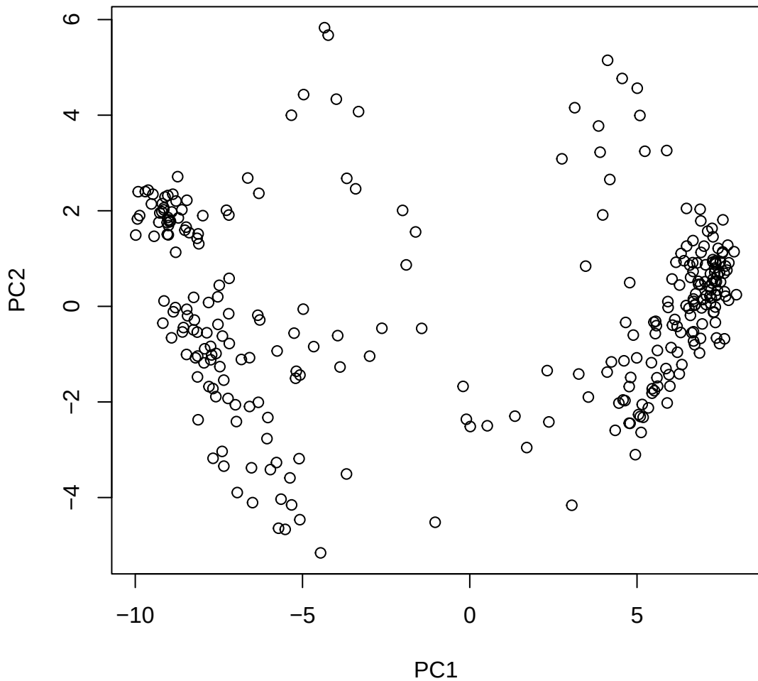
Window ID 220 NC_044057.1 (10)
