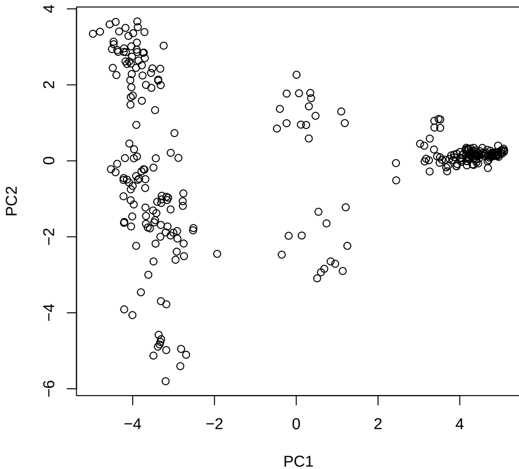
Window ID 242 NC_044058.1 (11)
