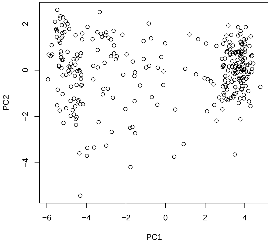
Window ID 243 NC_044058.1 (11)
