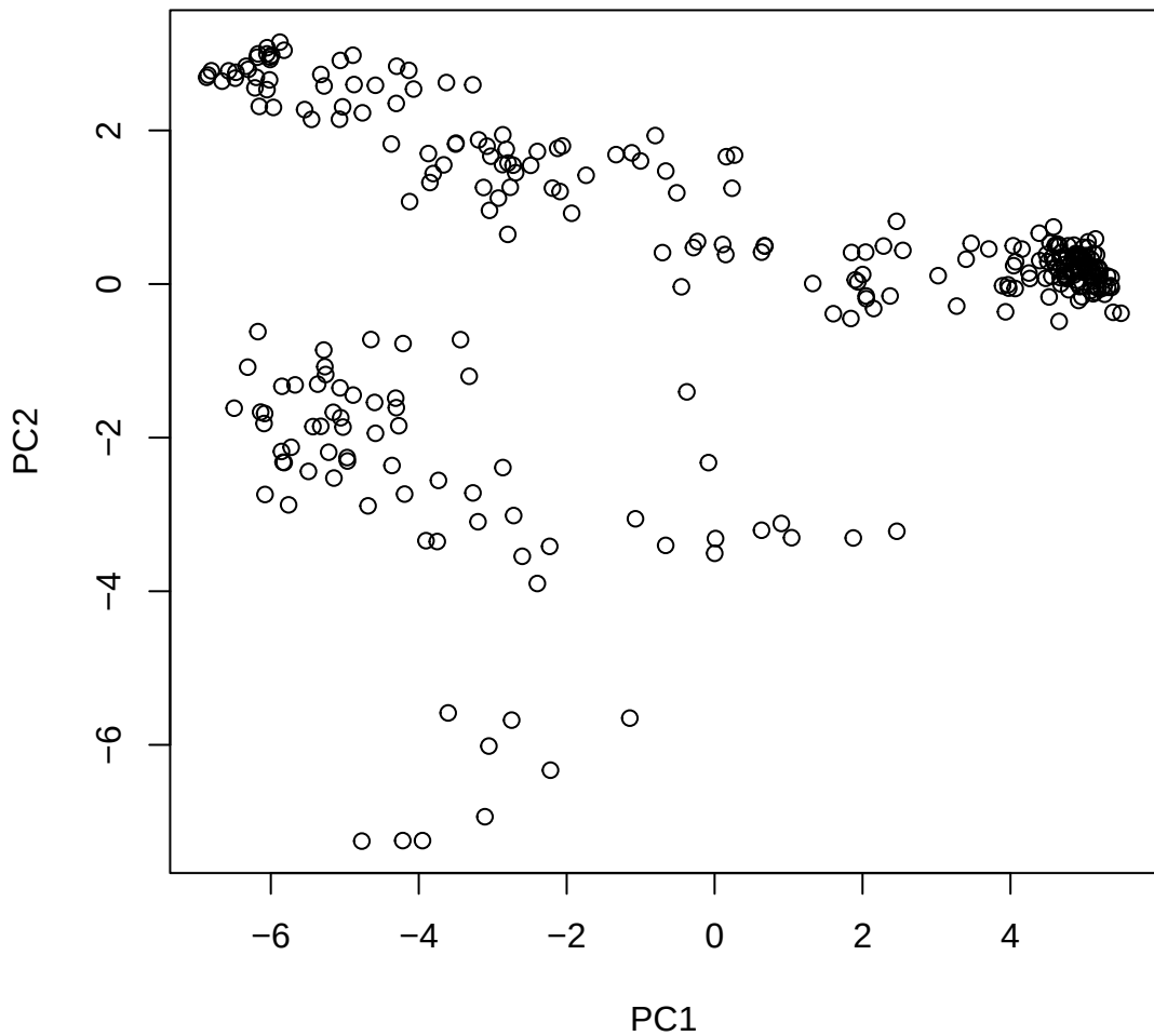
Window ID 244 NC_044058.1 (11)
