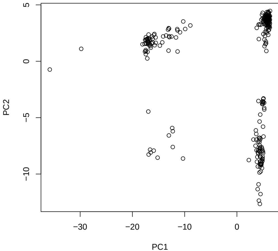
Window ID 252 NC_044058.1 (11)
