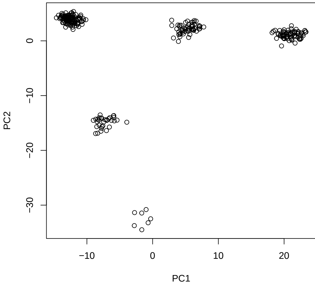
Window ID 258 NC_044059.1 (12)
