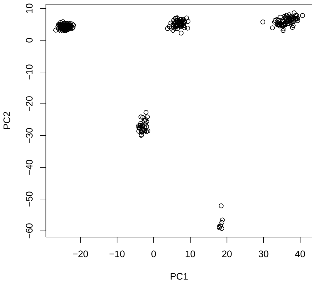
Window ID 271 NC_044059.1 (12)
