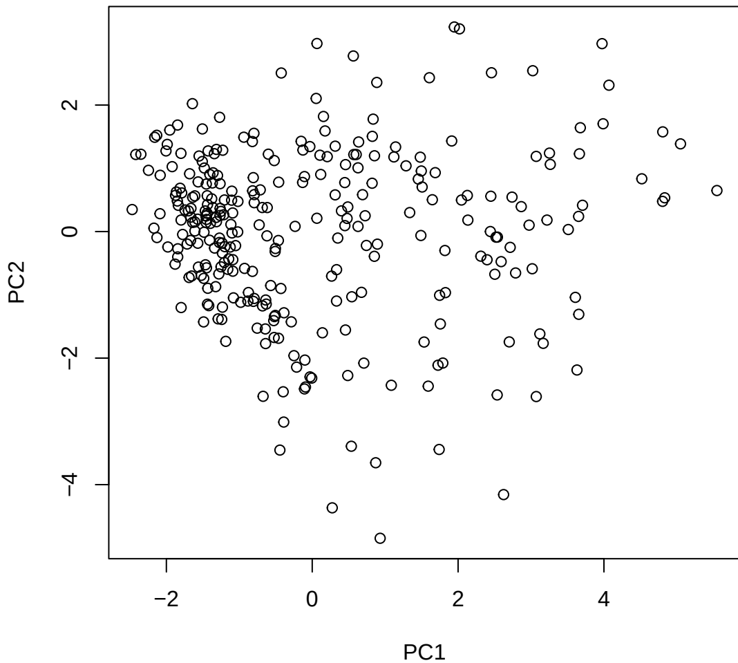
Window ID 280 NC_044060.1 (13)
