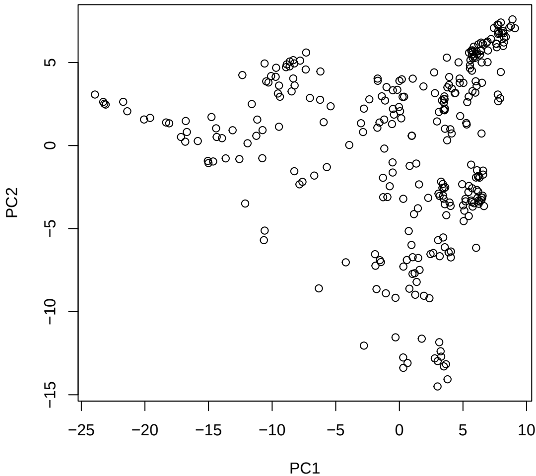
Window ID 290 NC_044060.1 (13)
