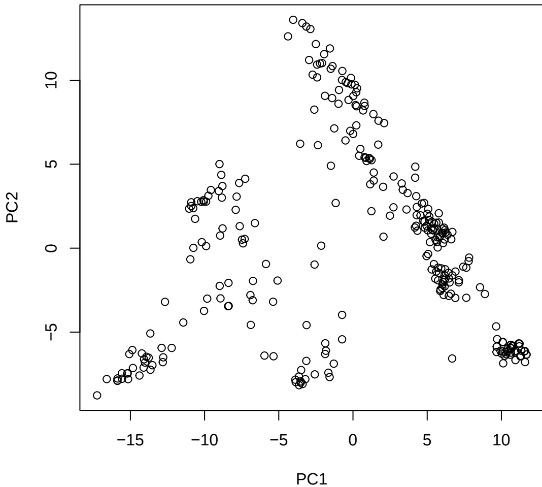
Window ID 294 NC_044061.1 (14)
