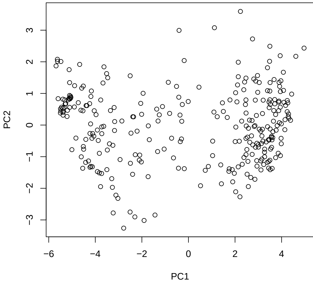
Window ID 297 NC_044061.1 (14)
