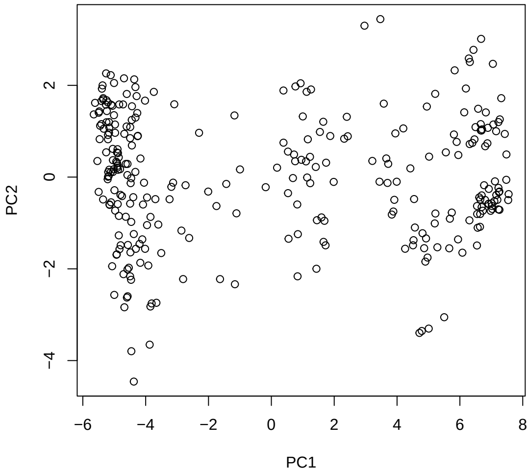
Window ID 302 NC_044061.1 (14)
