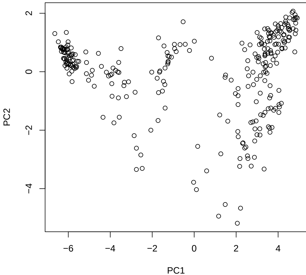
Window ID 309 NC_044061.1 (14)
