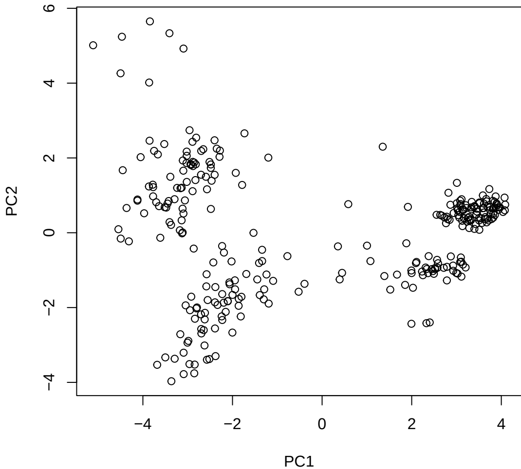
Window ID 321 NC_044062.1 (15)
