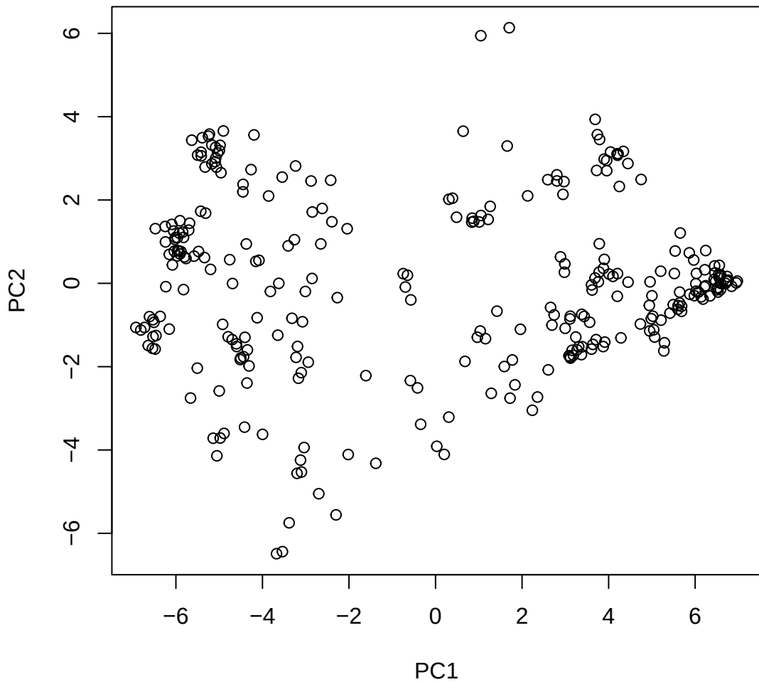
Window ID 323 NC_044062.1 (15)
