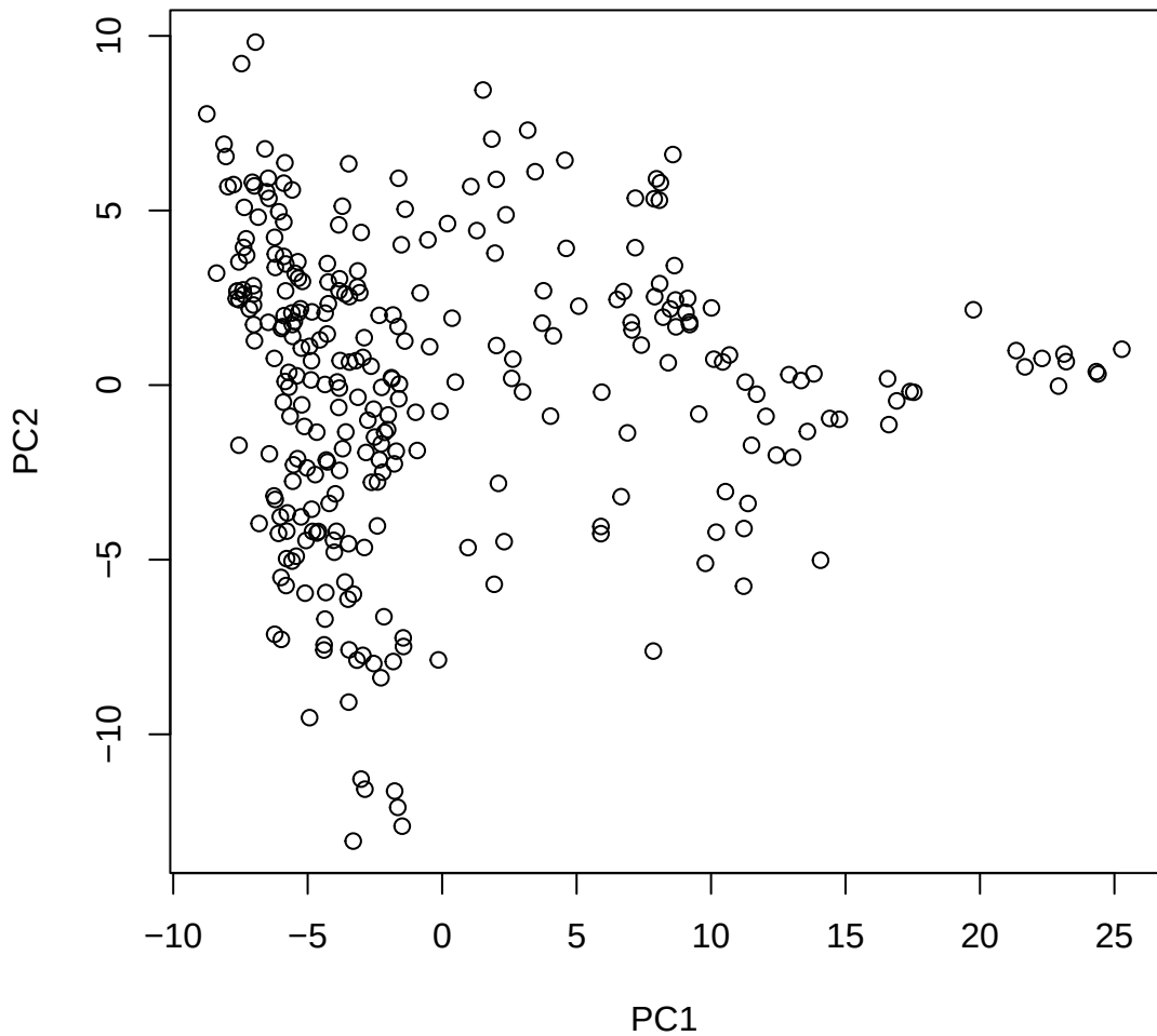
Window ID 331 NC_044062.1 (15)
