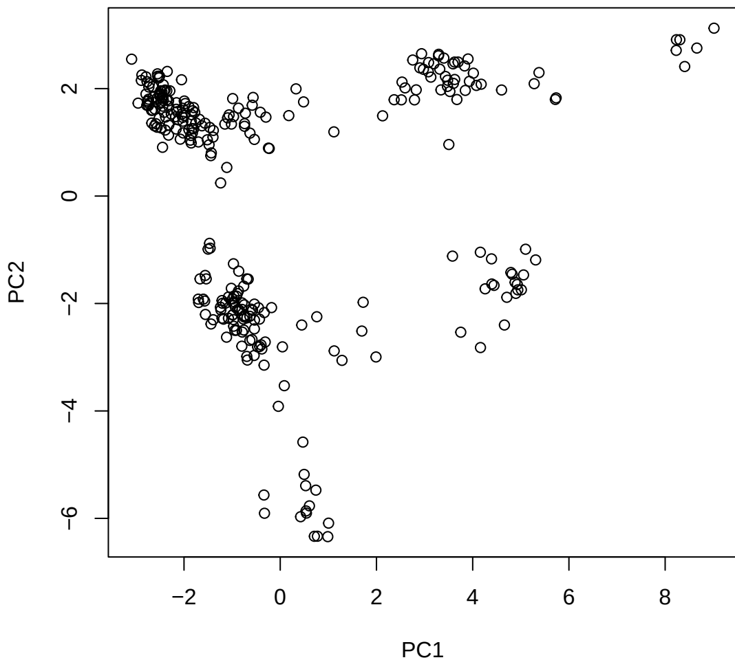
Window ID 357 NC_044063.1 (16)
