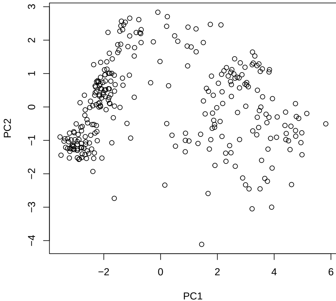
Window ID 399 NC_044066.1 (19)
