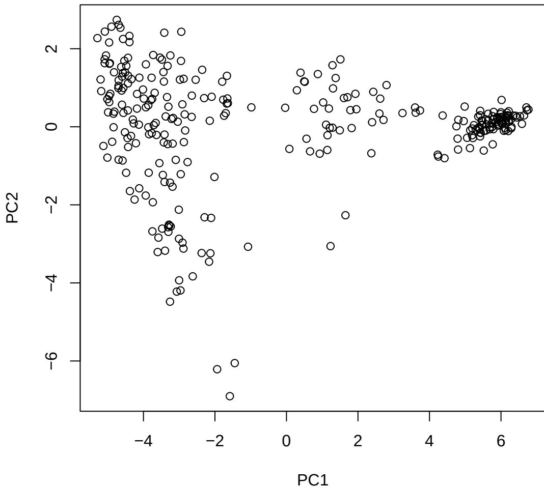
Window ID 404 NC_044067.1 (20)
