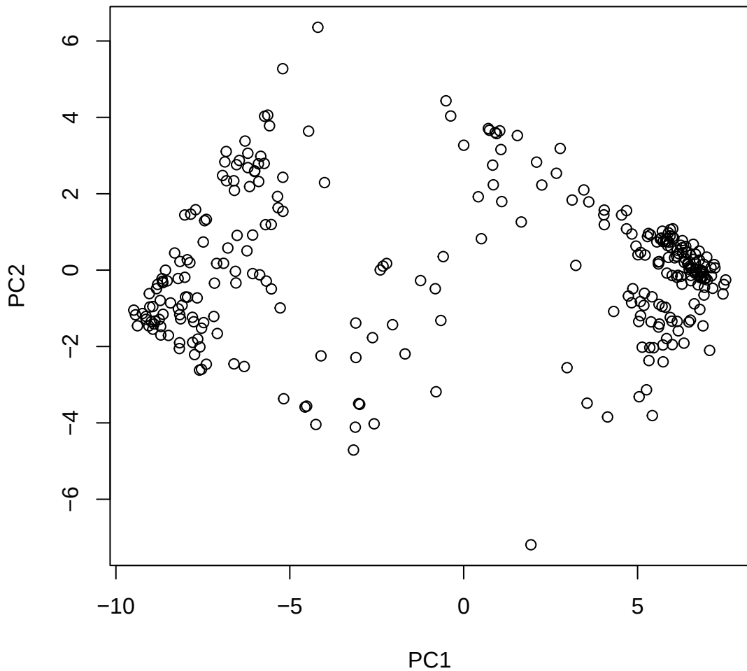
Window ID 407 NC_044067.1 (20)
