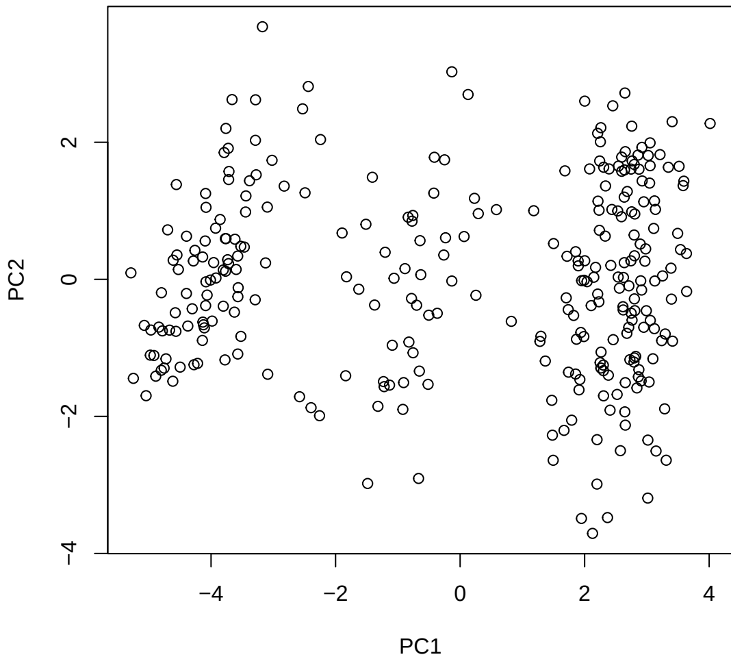
Window ID 416 NC_044068.1 (21)
