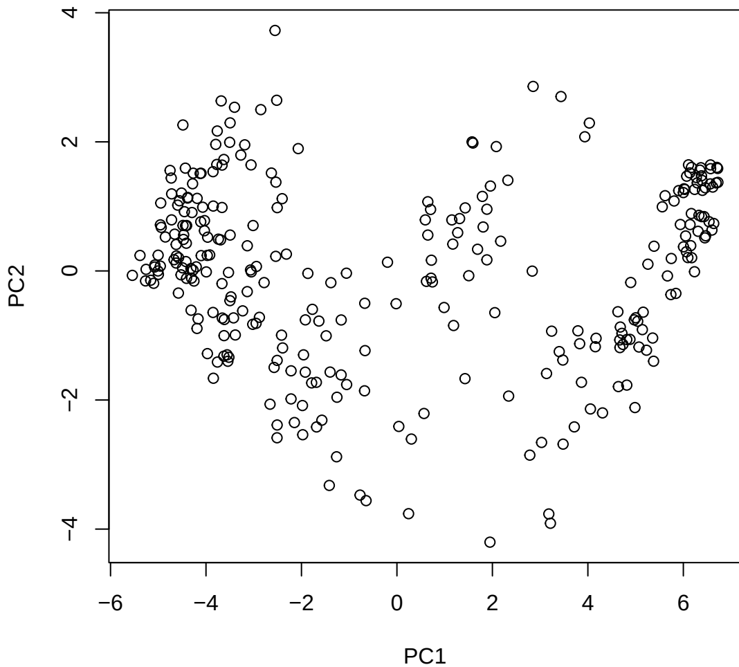
Window ID 422 NC_044068.1 (21)
