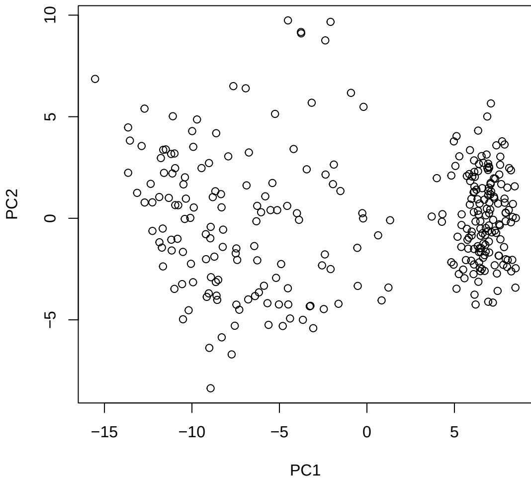
Window ID 8 NC_044049.1 (2)
