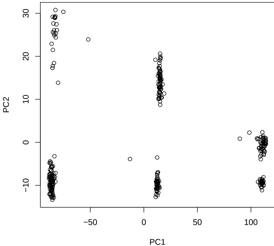
Window ID 9 NC_044049.1 (2)
