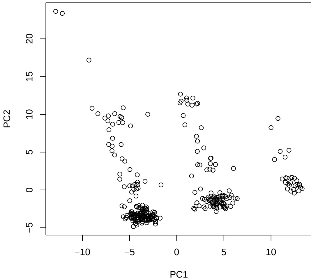
Window ID 29 NC_044050.1 (3)
