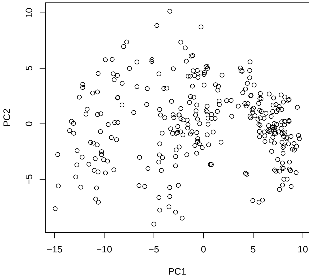
Window ID 31 NC_044050.1 (3)
