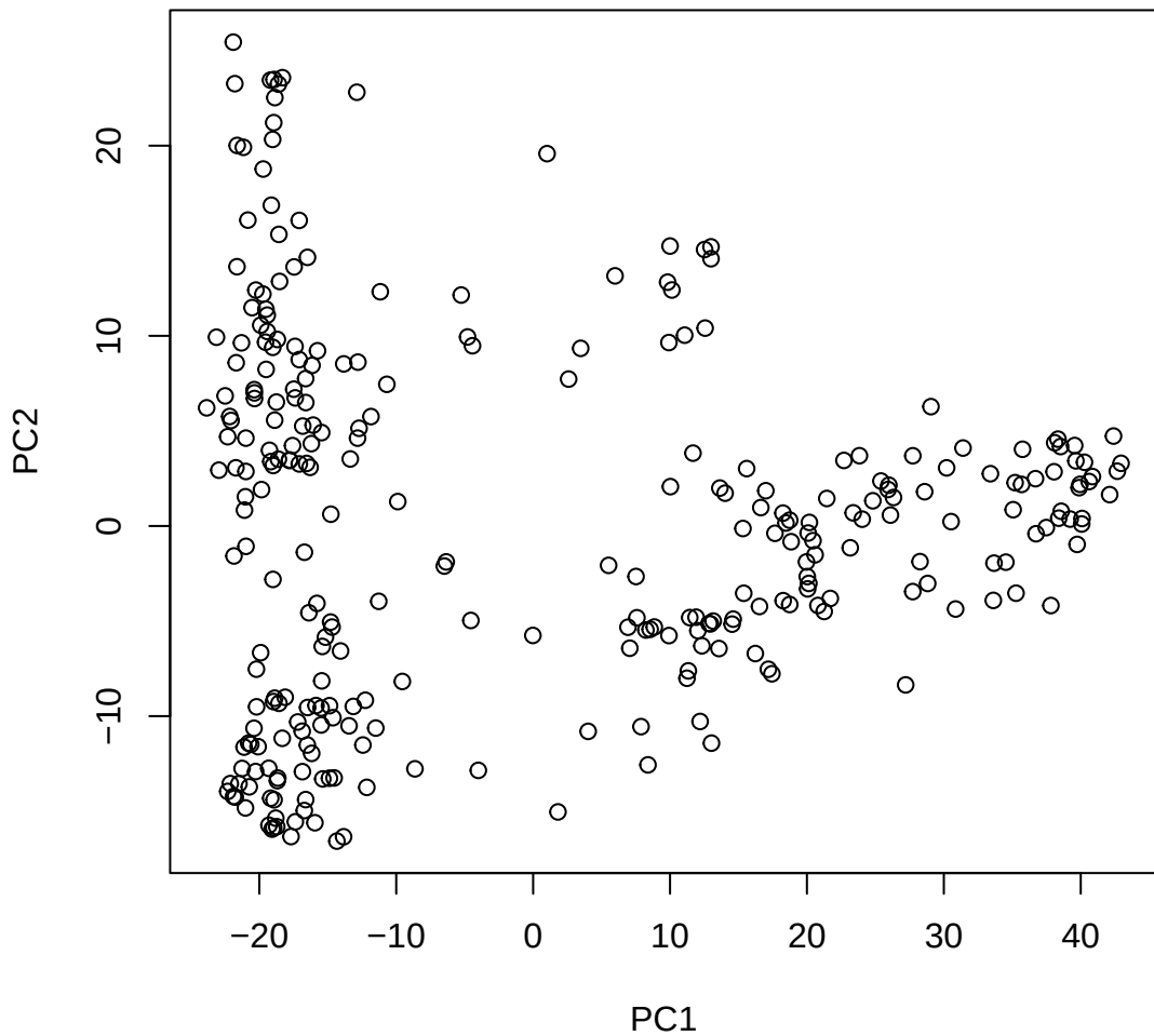
Window ID 92 NC_044056.1 (9)
