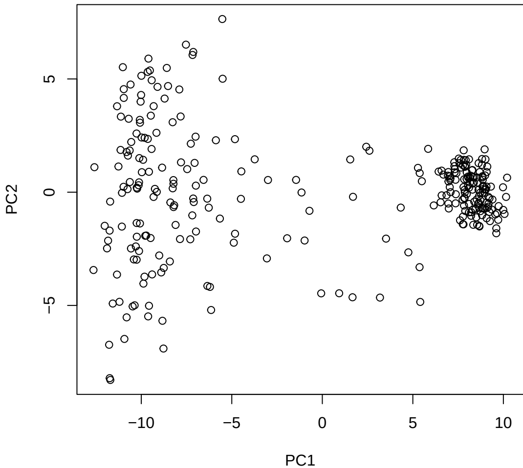
Window ID 125 NC_044061.1 (14)
