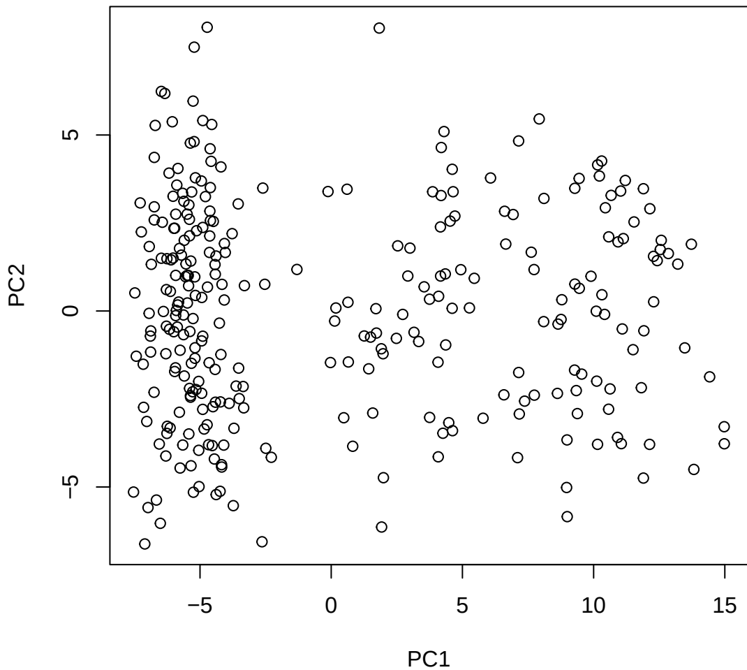
Window ID 180 NC_044067.1 (20)
