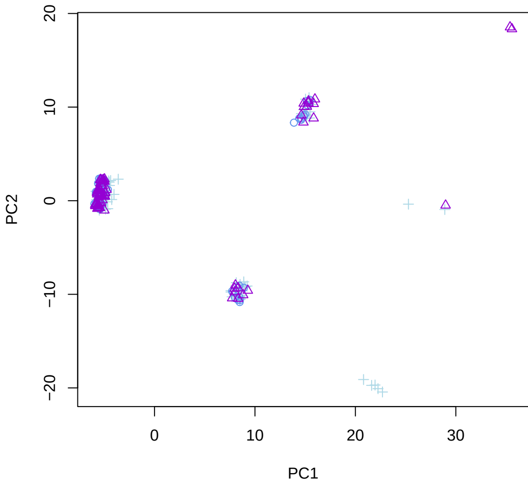
WindowID: 6; NC_044048.1 (LG 1); 999 SNPs
