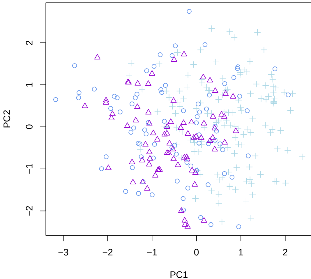
WindowID: 99; NC_044051.1 (LG 4); 99 SNPs
