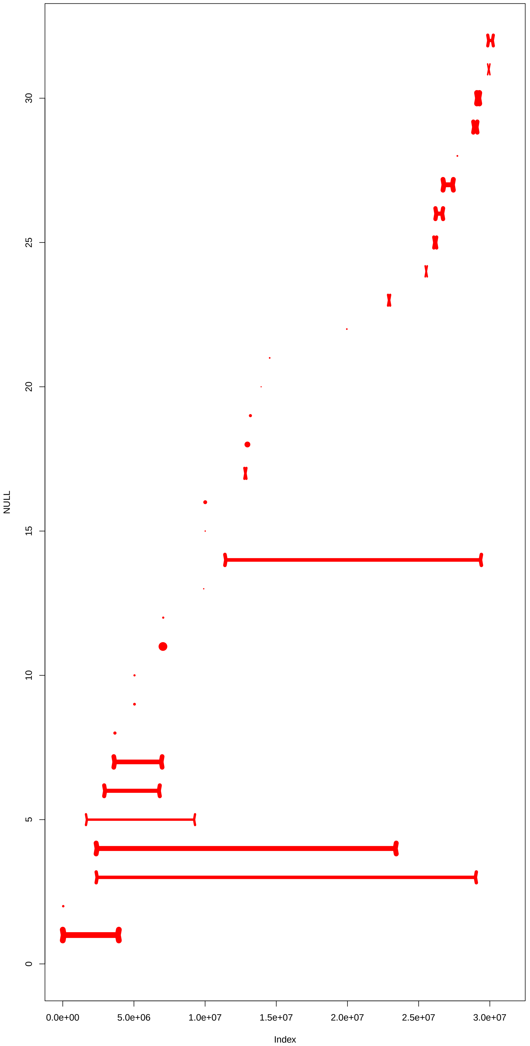
NC_044050.1 pass2
