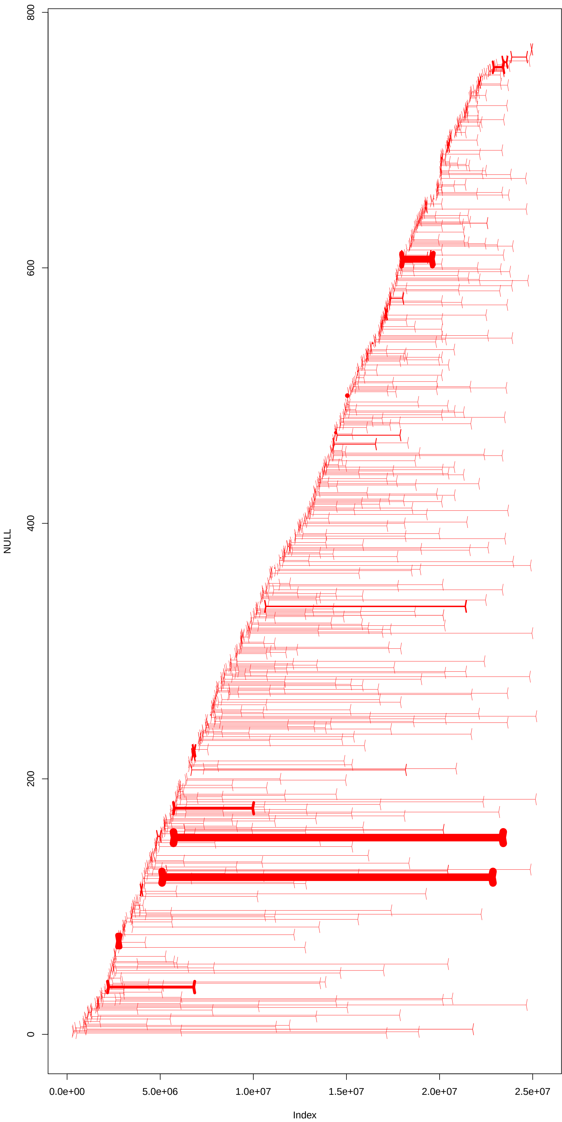
NC_044052.1
