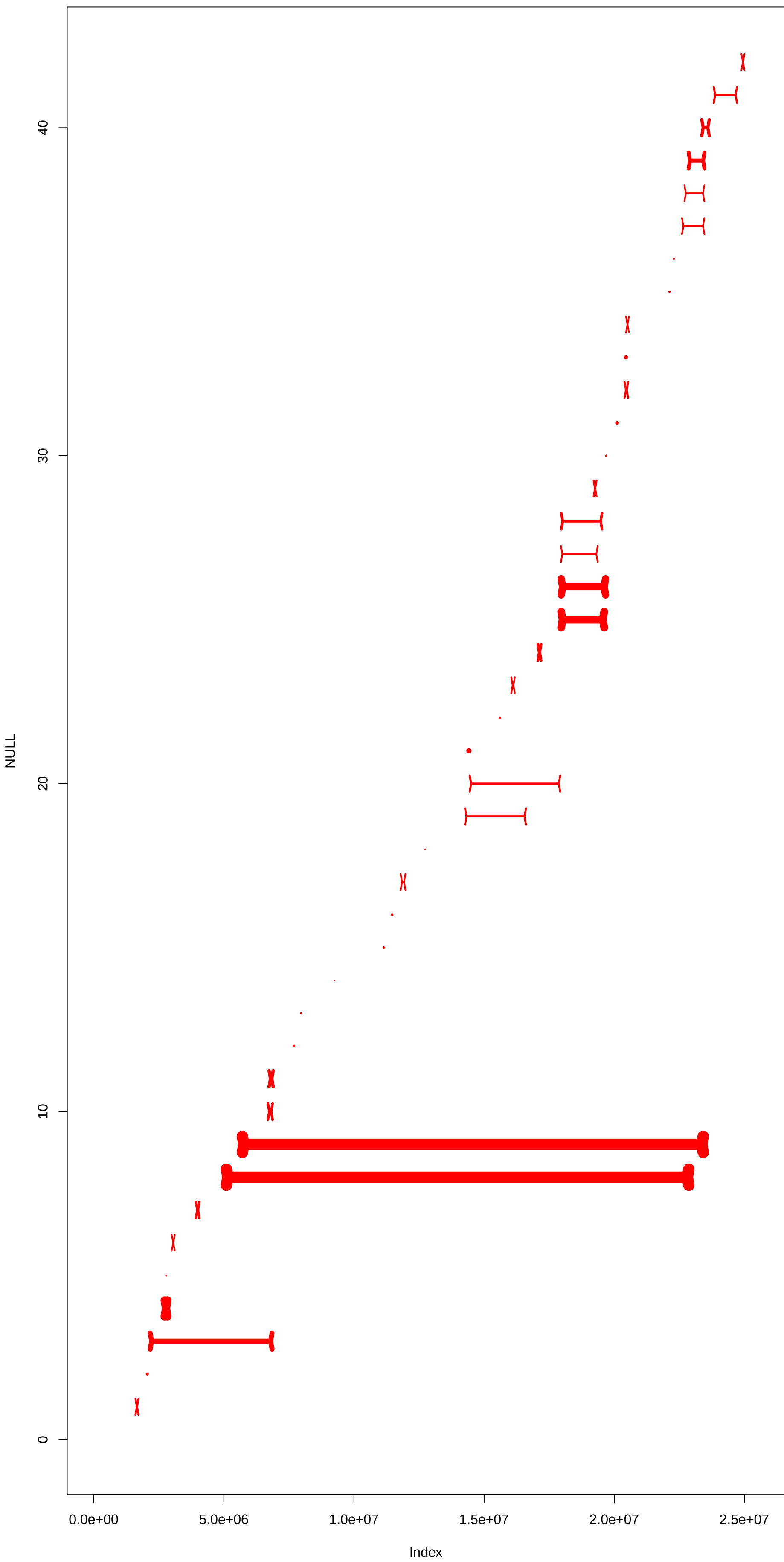
NC_044052.1 pass1
